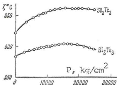
Melting curves of \text{Bi}_2\text{Te}_3 and \text{Sb}_2\text{Te}_3 up to 25000 \text{kg/cm}^2
